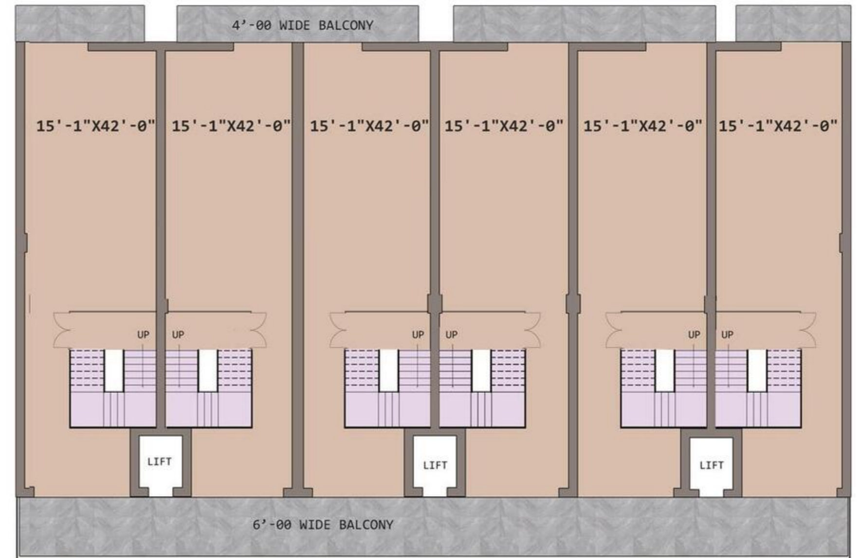
SECOND & THIRD FLOOR PLAN
