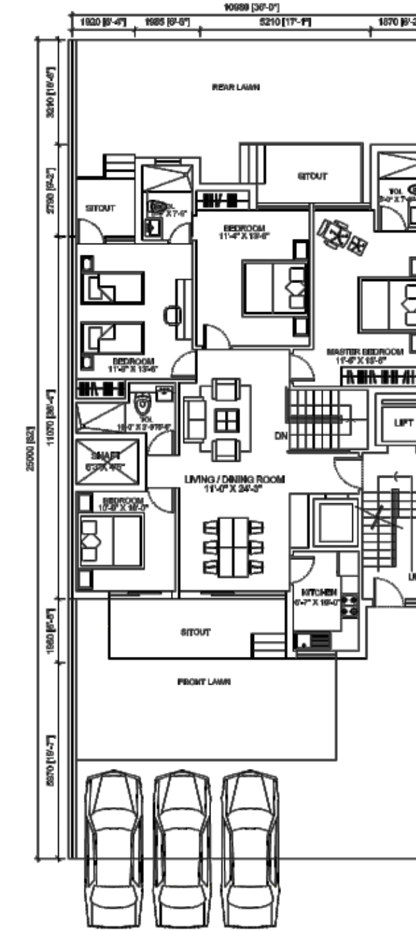
Ground Floor Plan 168.95sq mt. (1818 sq ft.)
