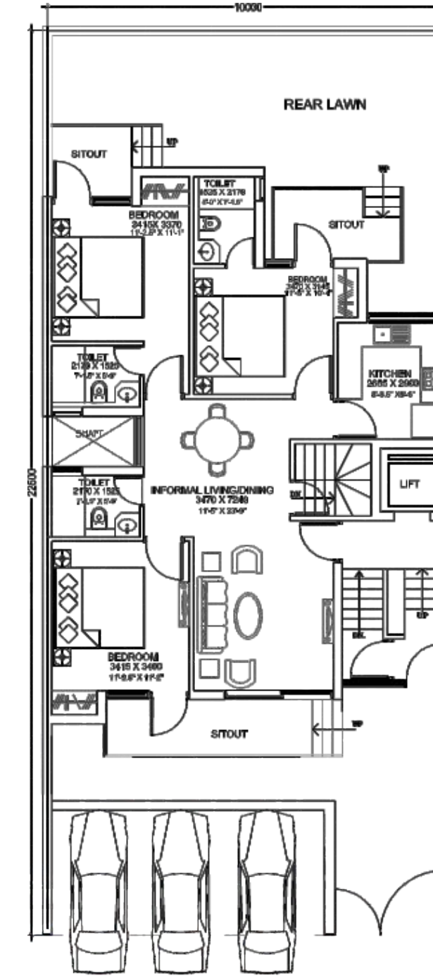
Ground Floor Plan 145 sq mt. (1561 sq ft.)
